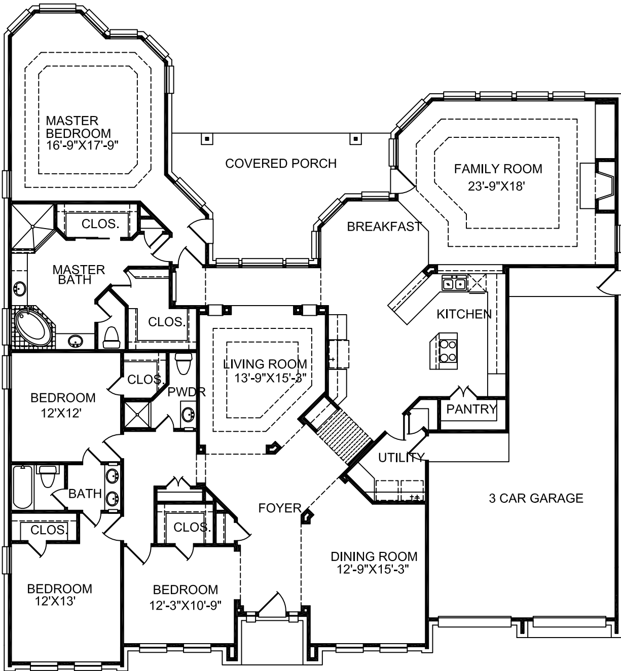
FIRST FLOOR
