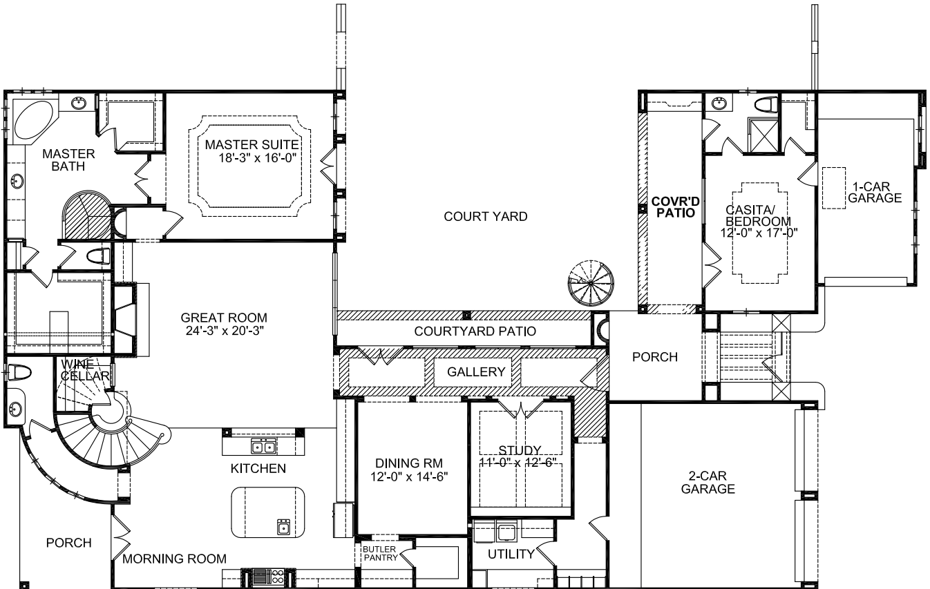
FIRST FLOOR
