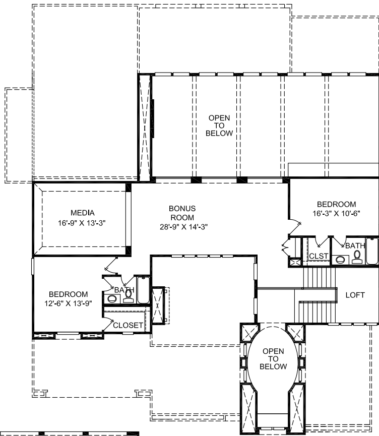
SECOND FLOOR
