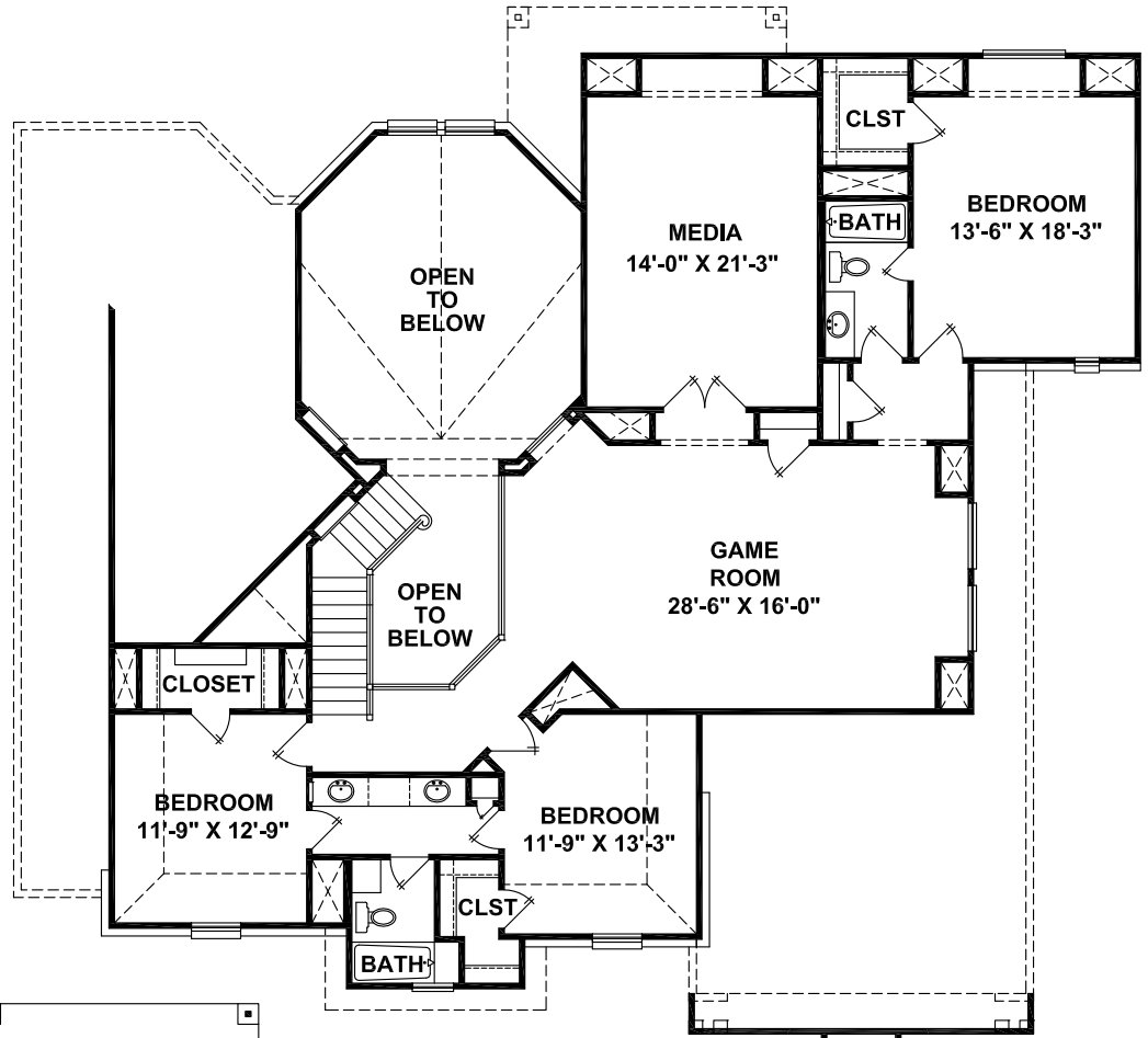
SECOND FLOOR
