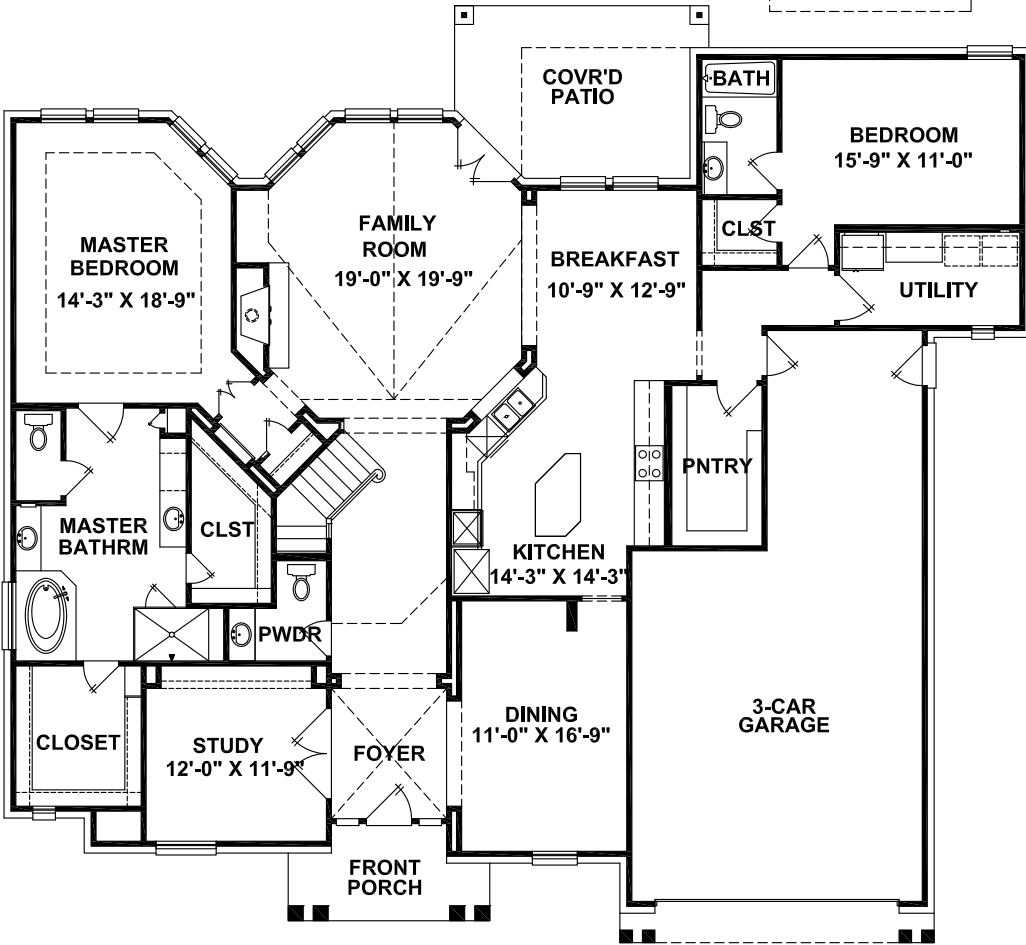
FIRST FLOOR
