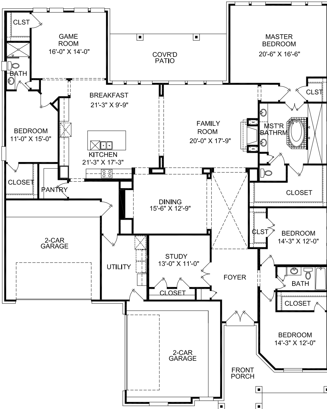
FIRST FLOOR
