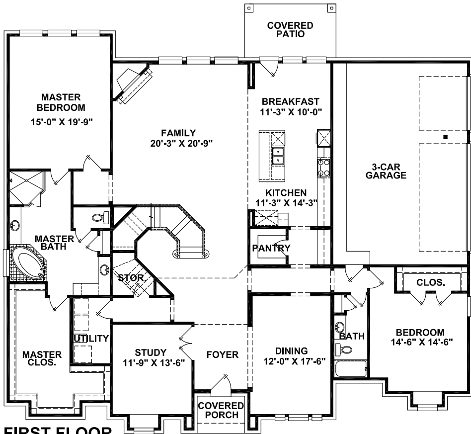
FIRST FLOOR
