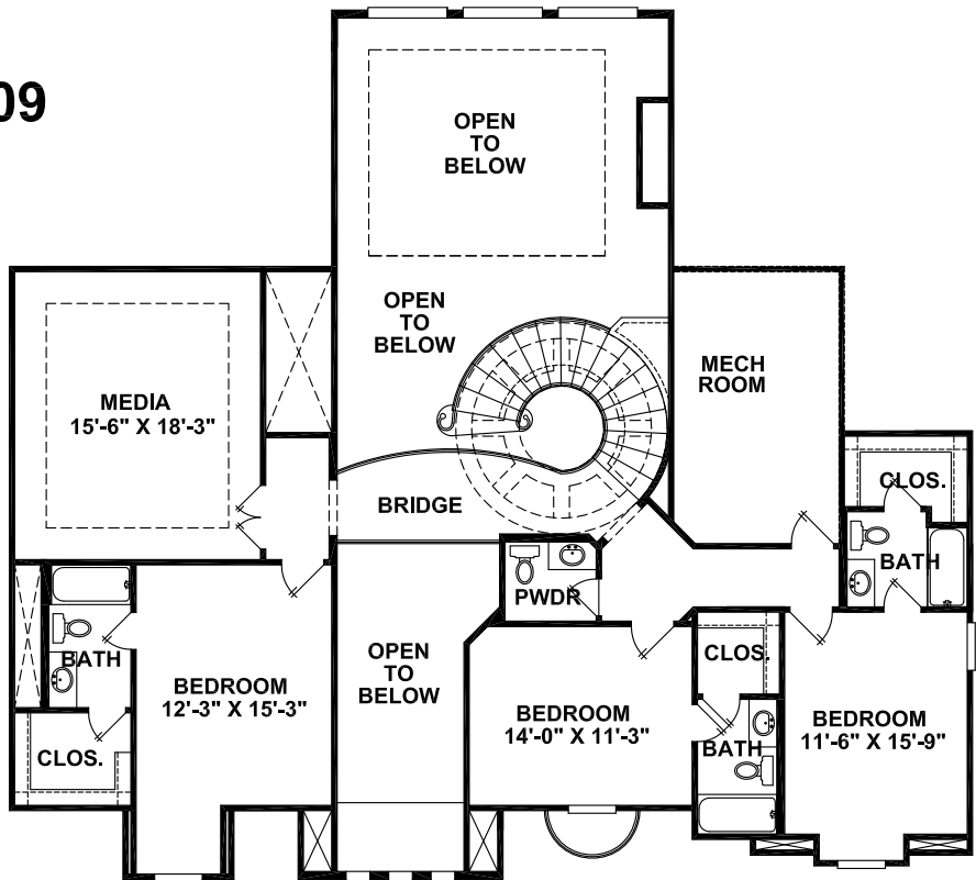
SECOND FLOOR
