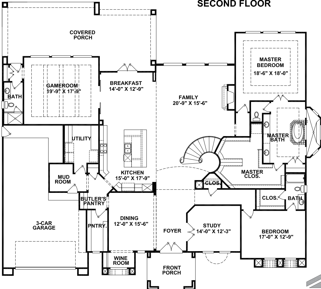
SECOND FLOOR
