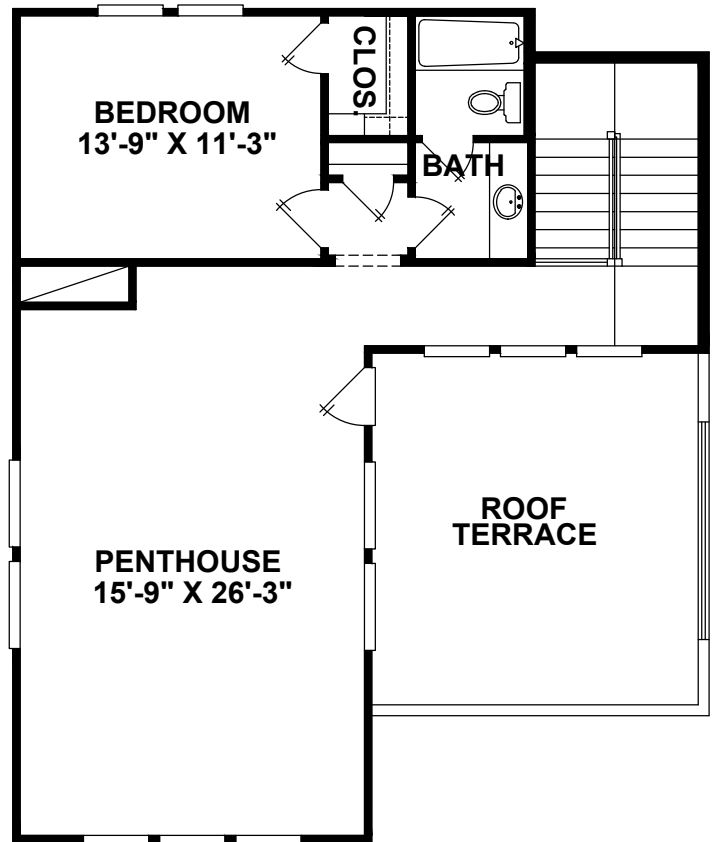
THIRD FLOOR
