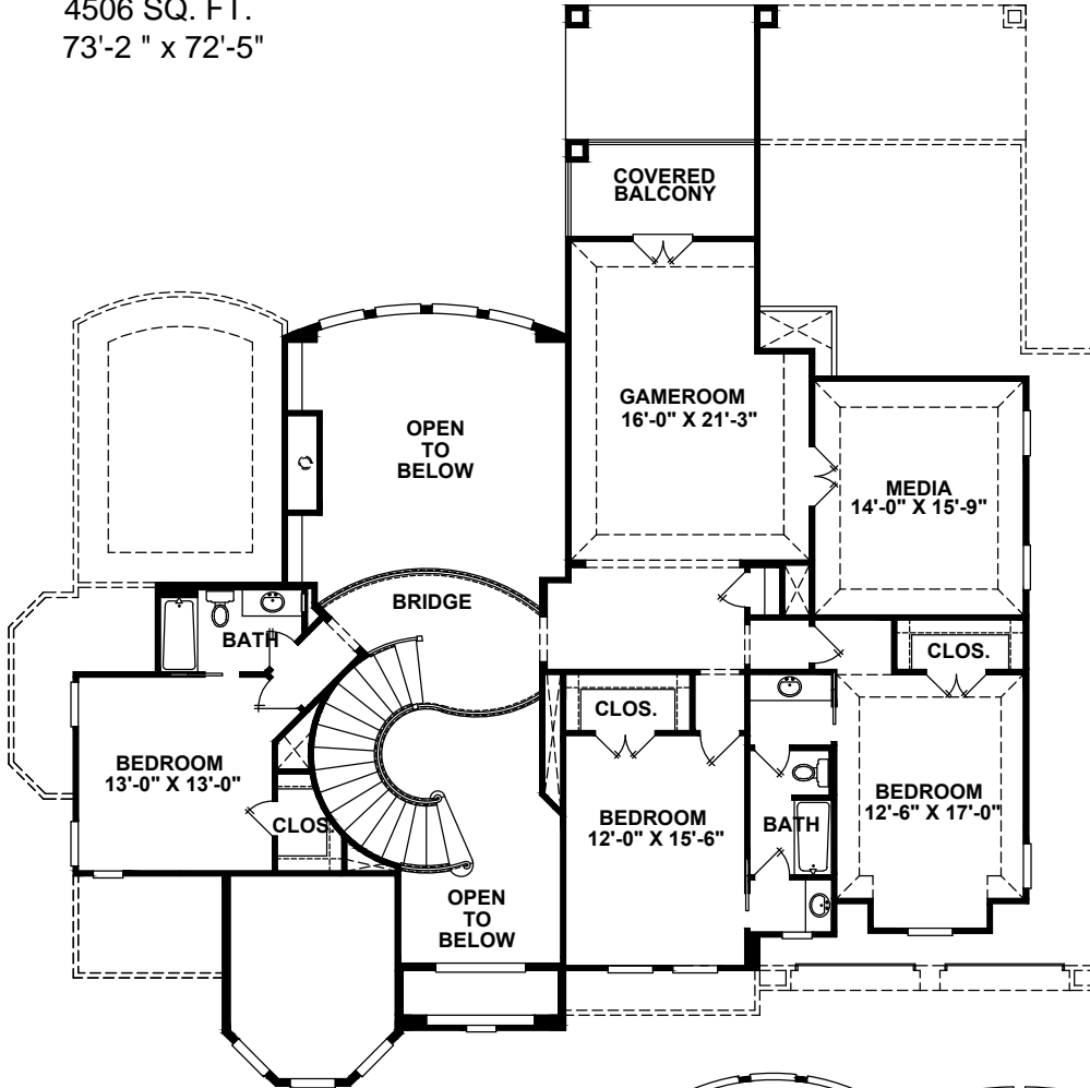
SECOND FLOOR
