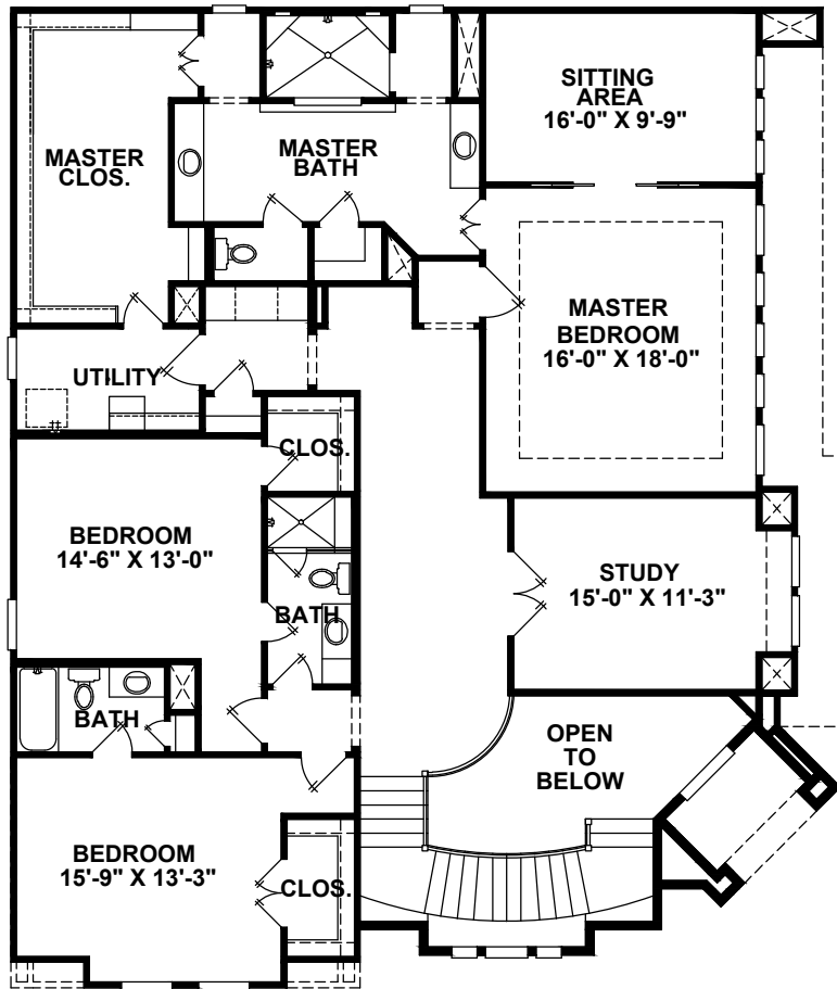
SECOND FLOOR
