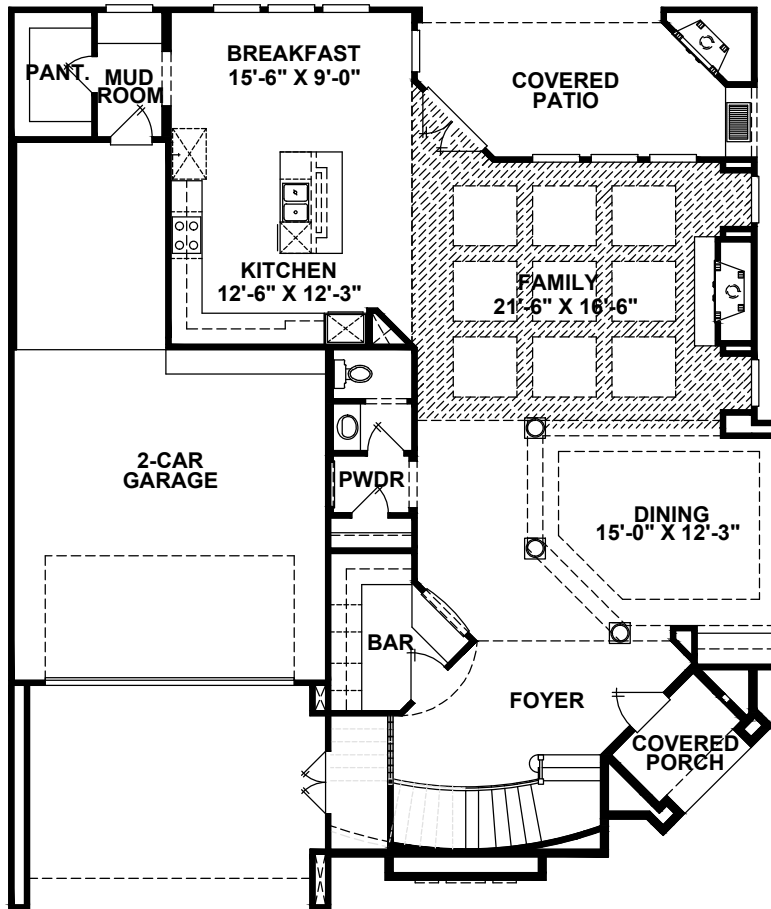
FIRST FLOOR
