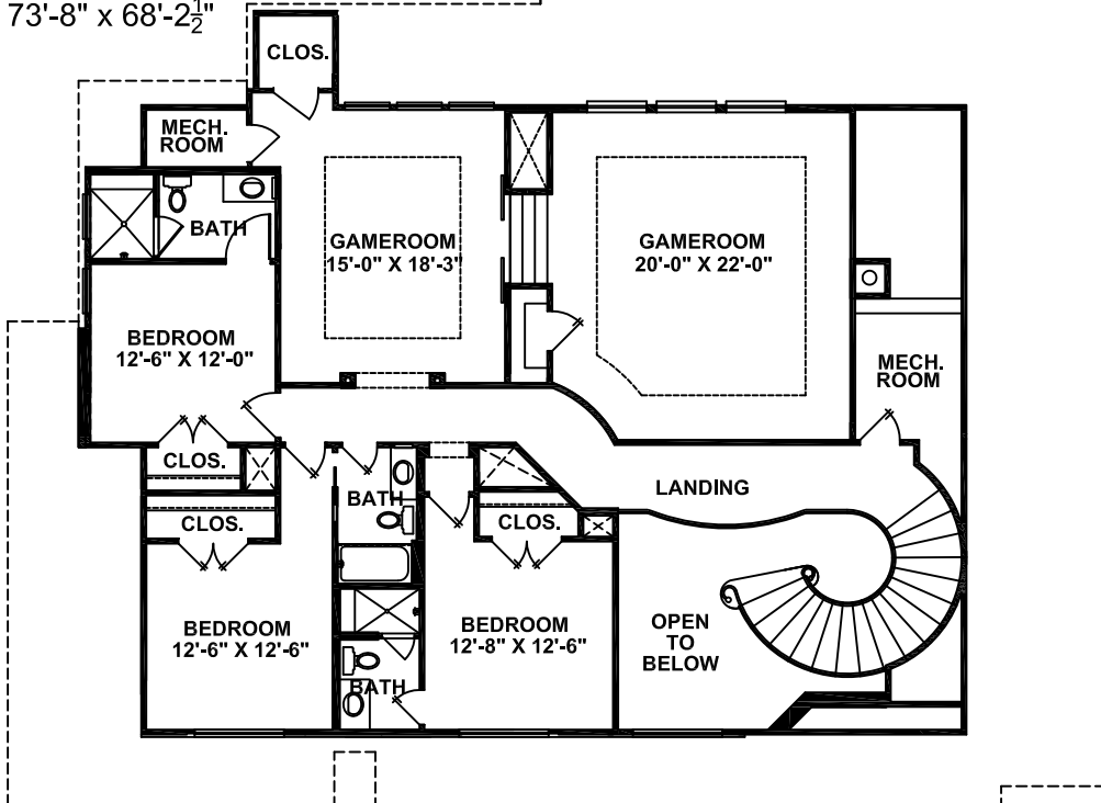
SECOND FLOOR
