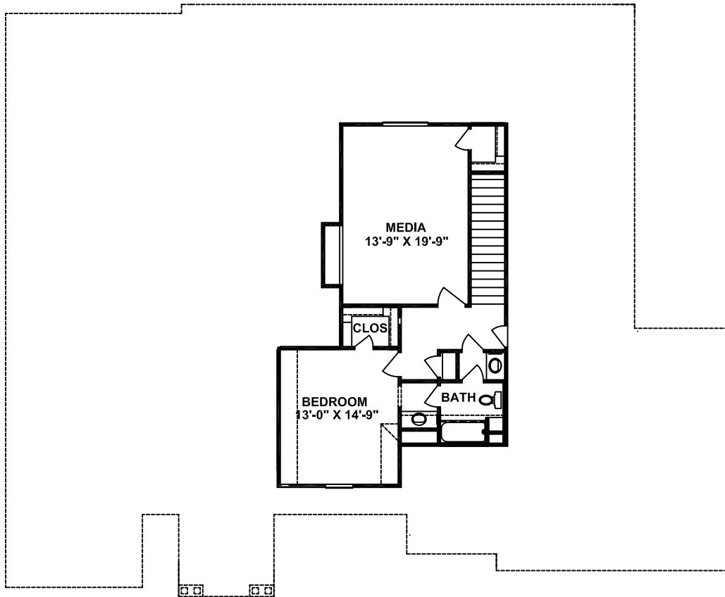
SECOND FLOOR
