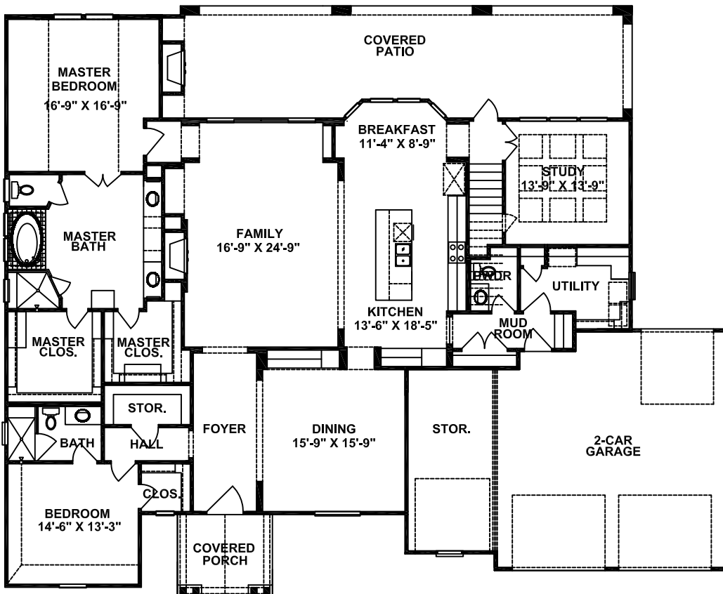
FIRST FLOOR
