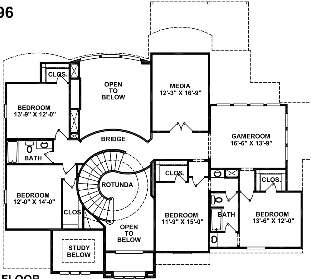
SECOND FLOOR
