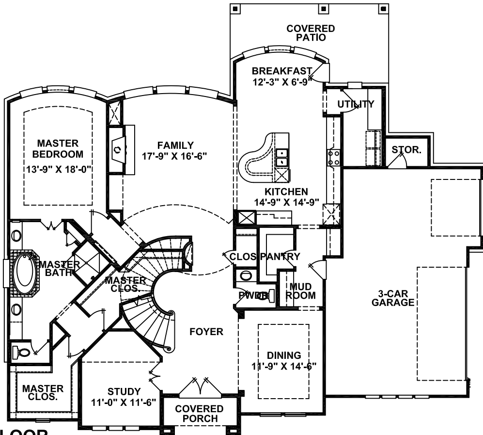
FIRST FLOOR
