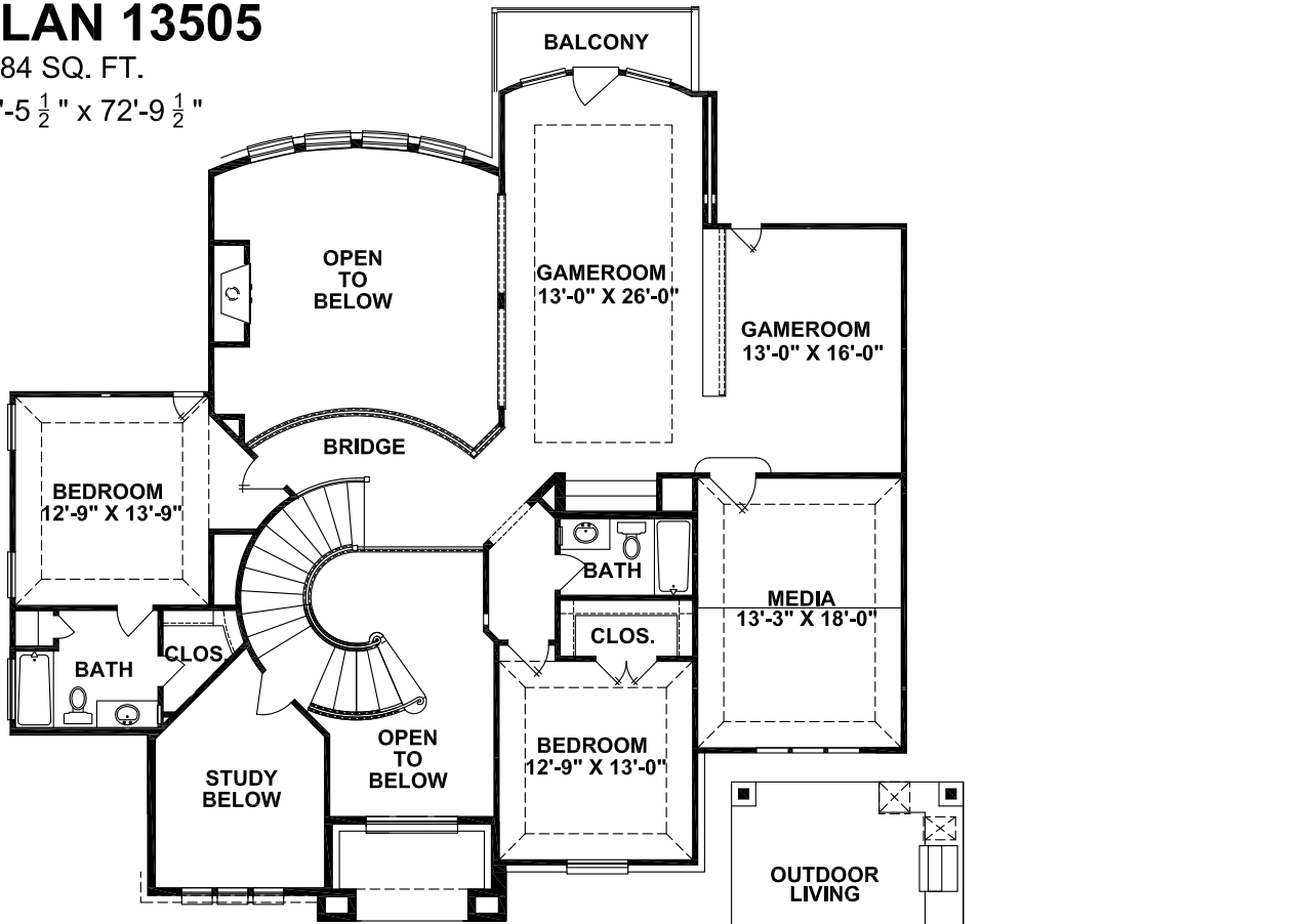
SECOND FLOOR
