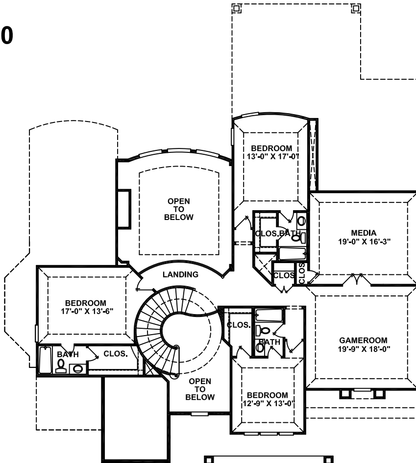
SECOND FLOOR
