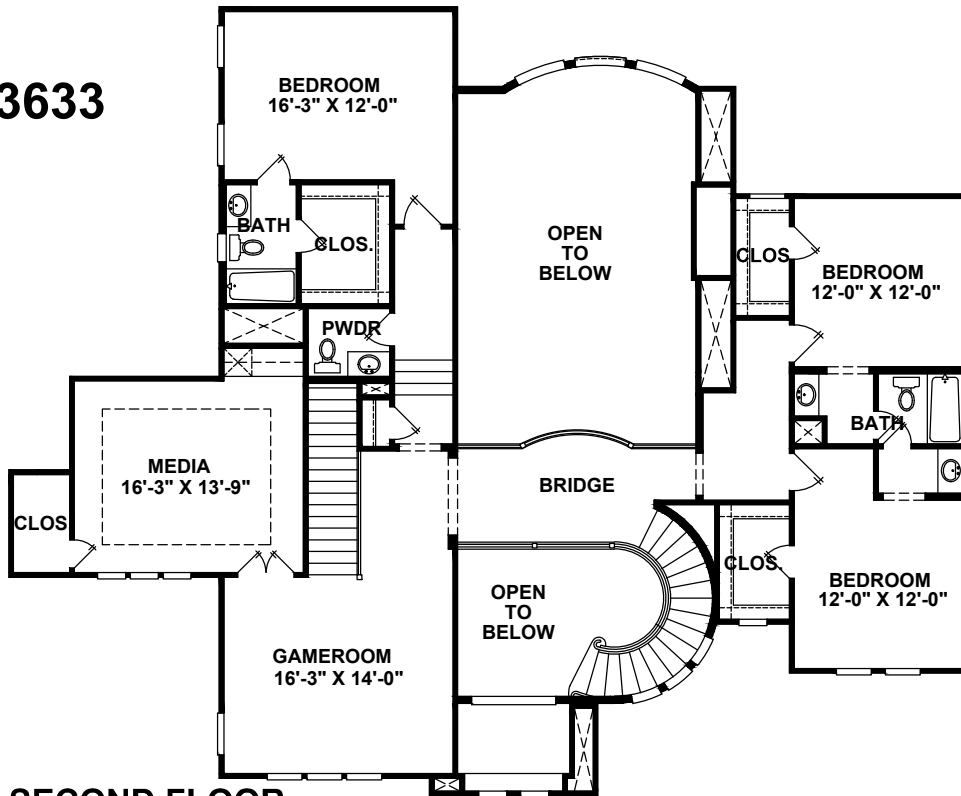
SECOND FLOOR
