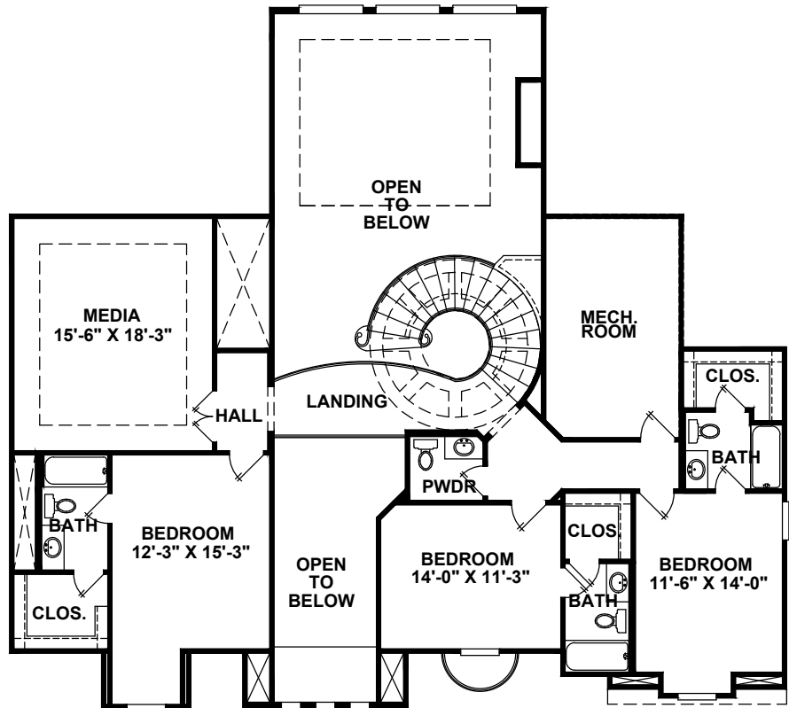
SECOND FLOOR
