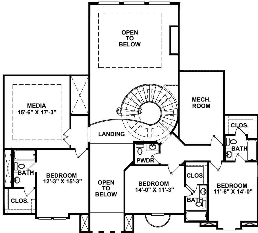
SECOND FLOOR
