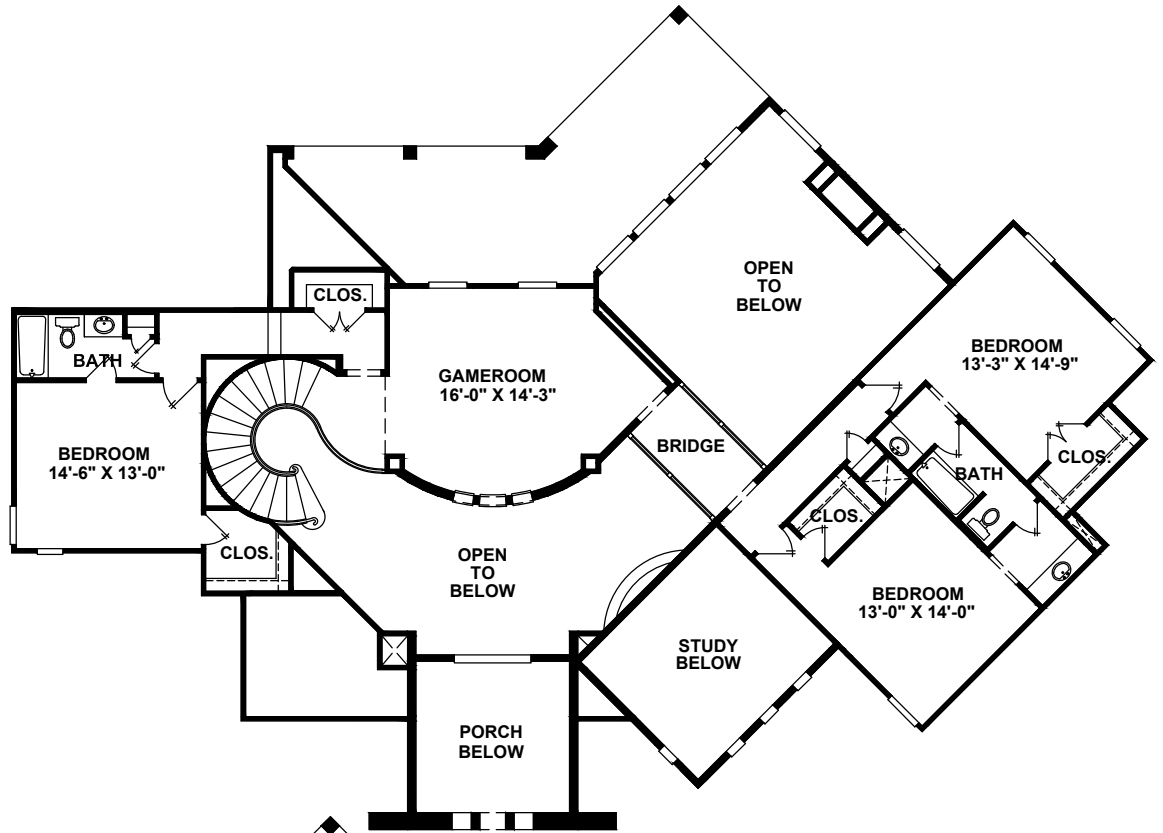
SECOND FLOOR
