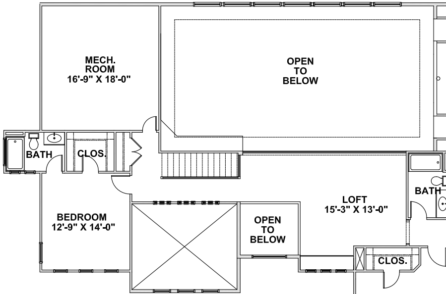
SECOND FLOOR
