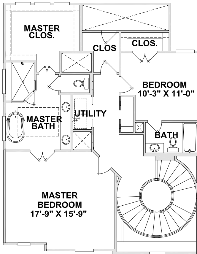
THIRD FLOOR
