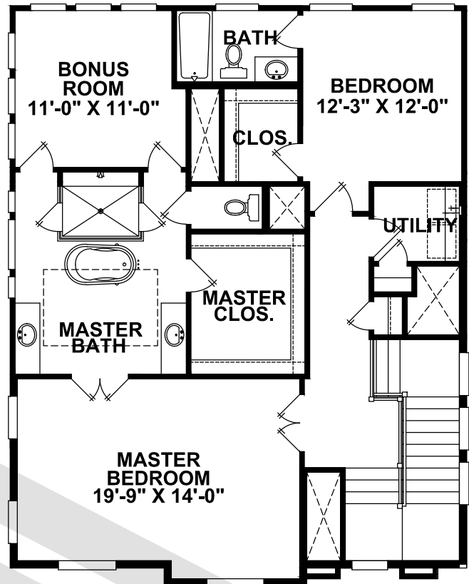
THIRD FLOOR
