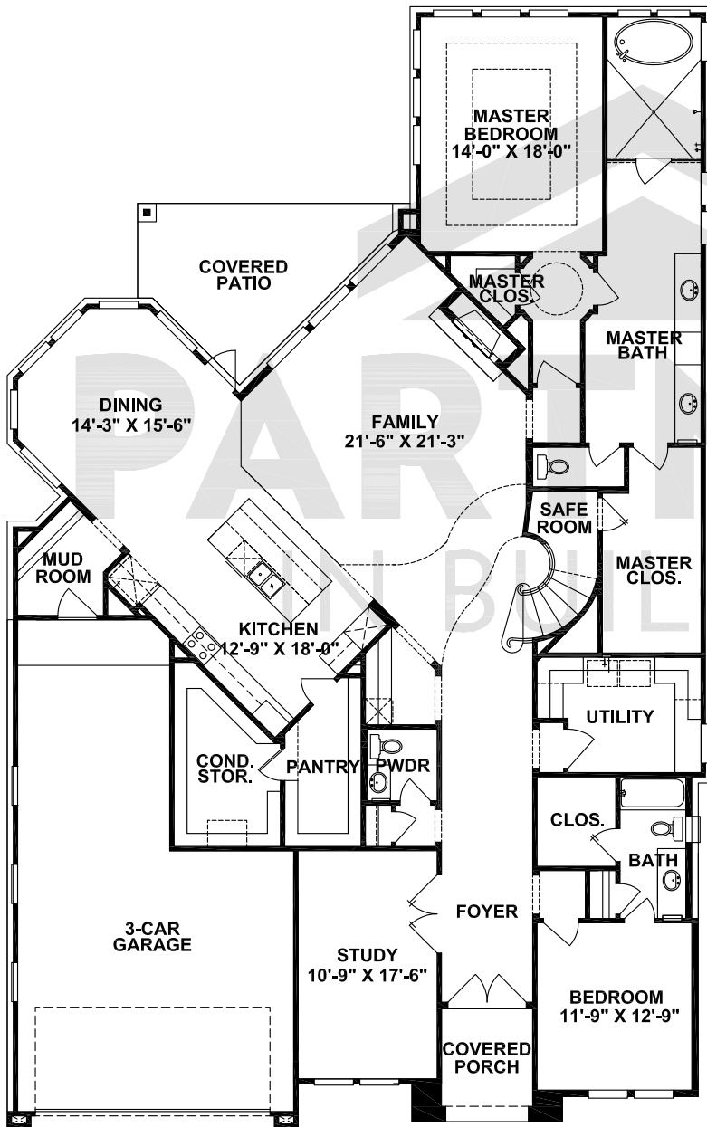
FIRST FLOOR
