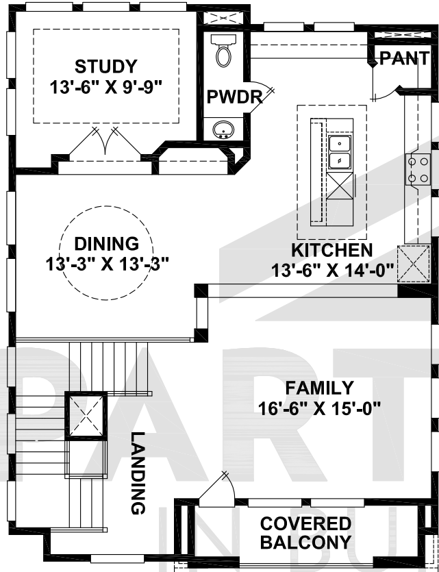
SECOND FLOOR
