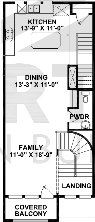
SECOND FLOOR
