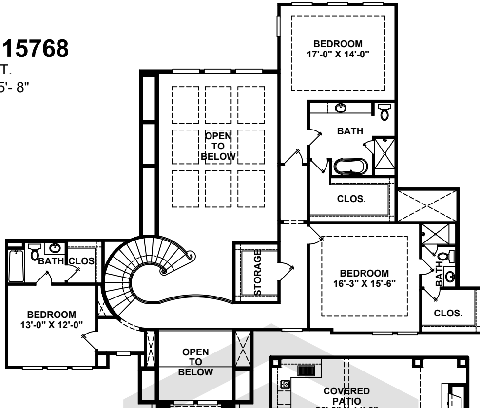
SECOND FLOOR
