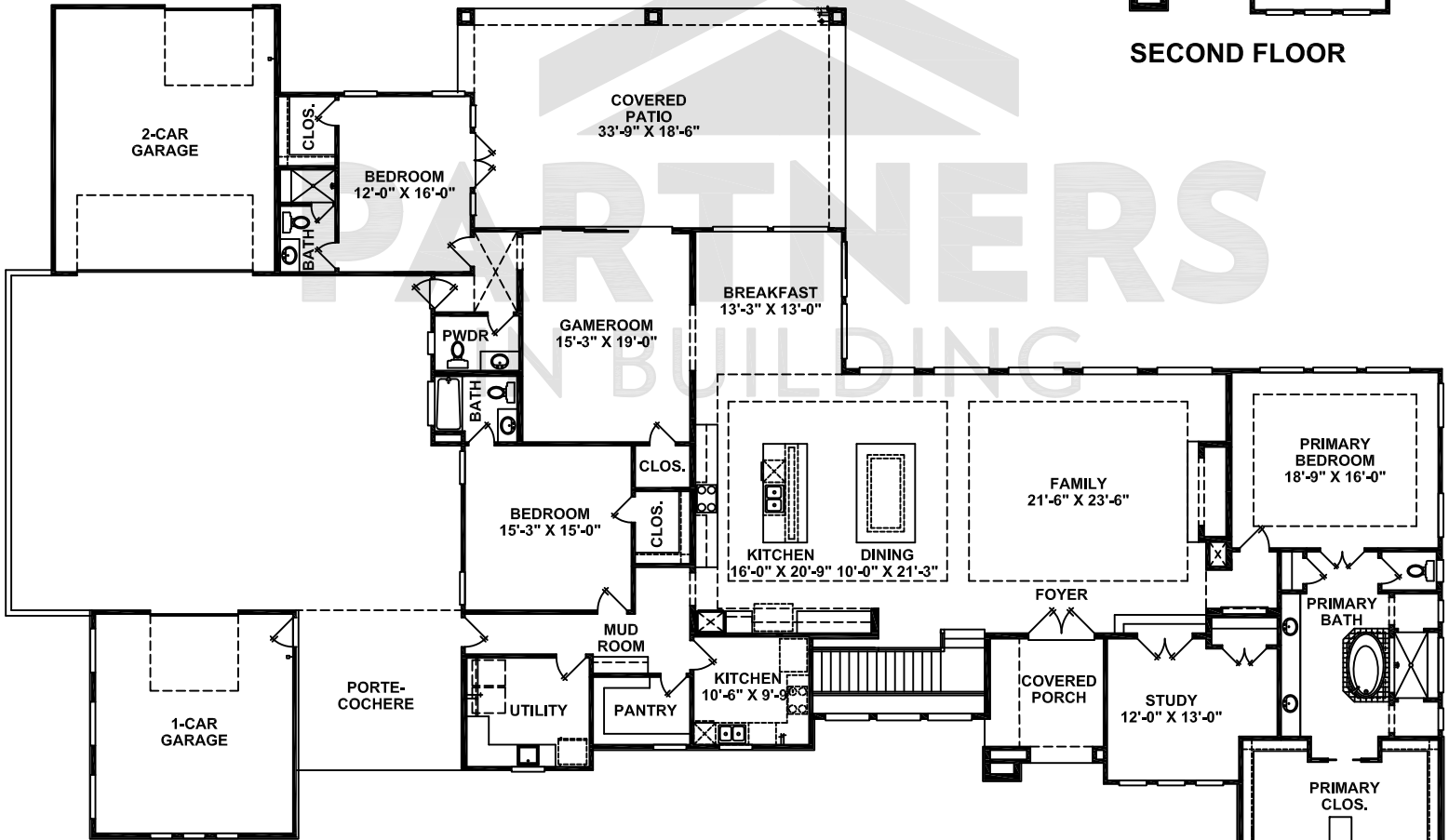
FIRST FLOOR
