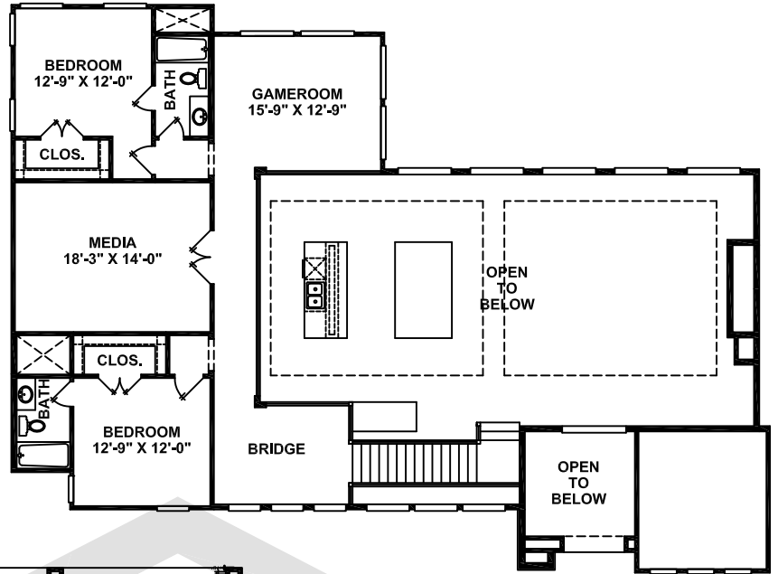
SECOND FLOOR
