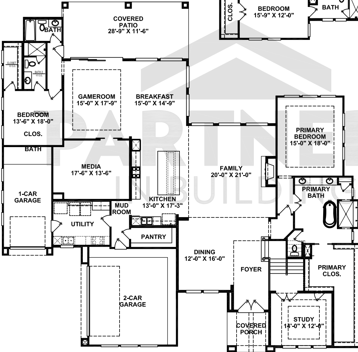
FIRST FLOOR
