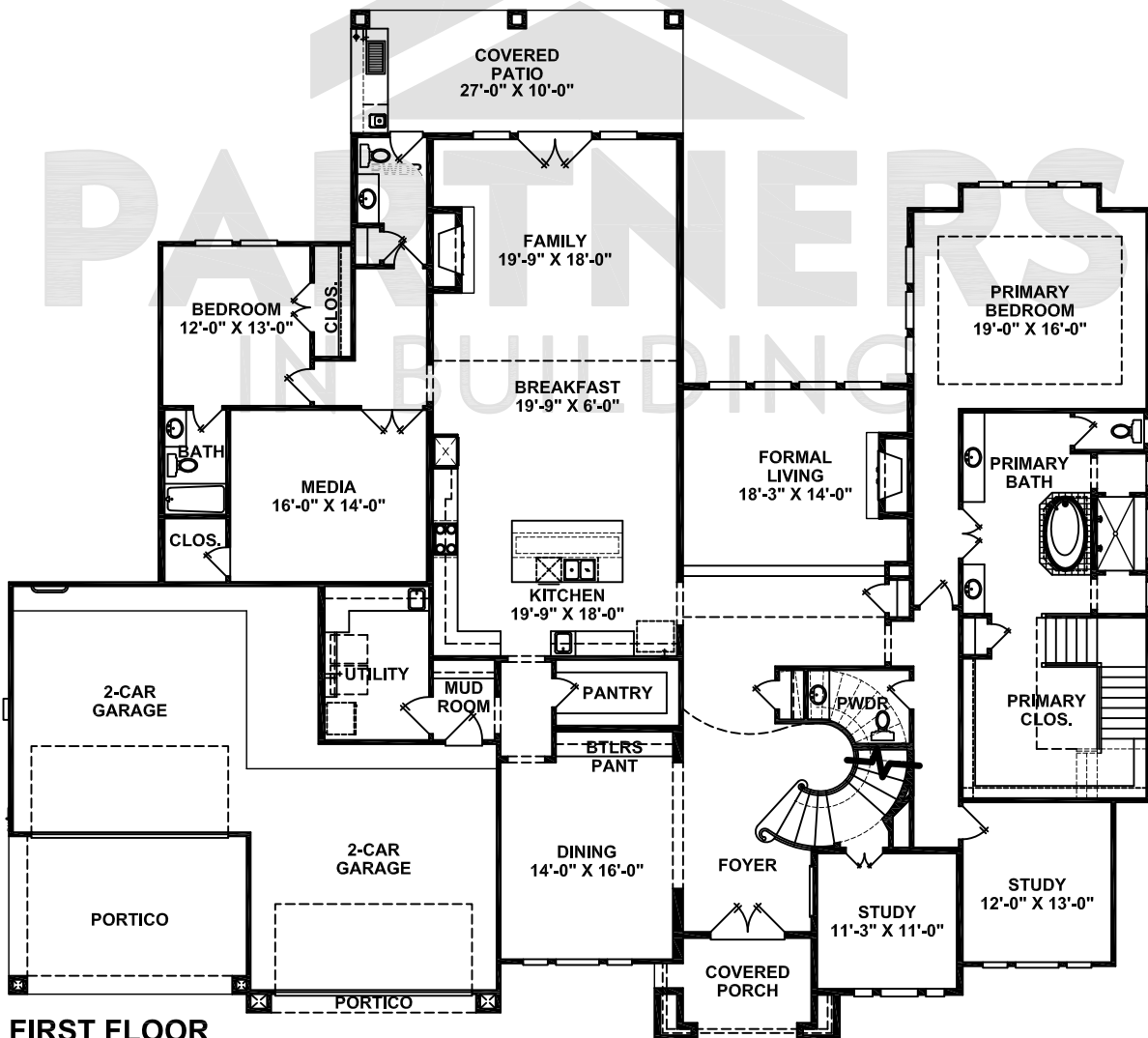
FIRST FLOOR
