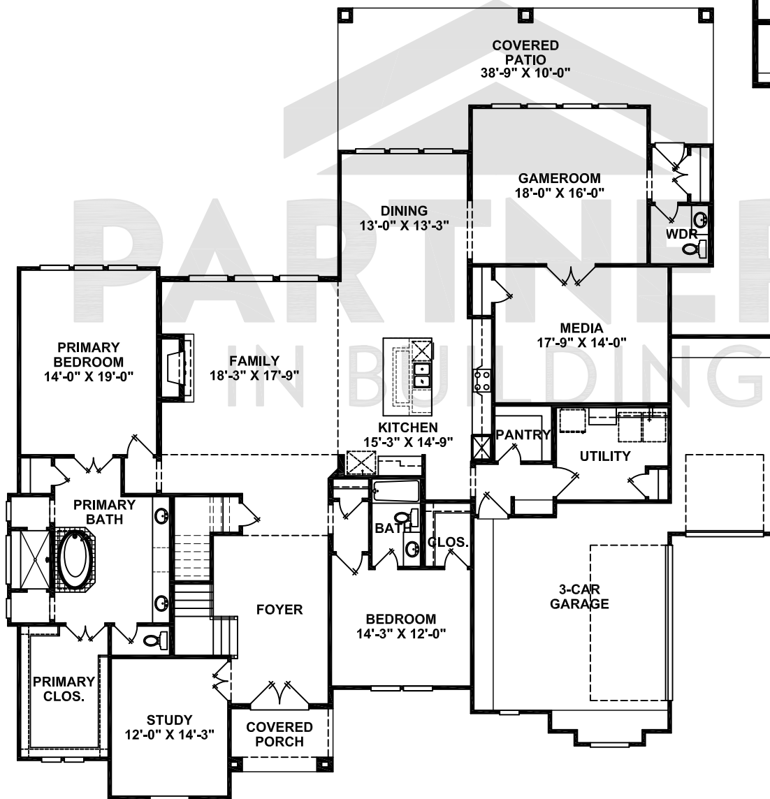
FIRST FLOOR
