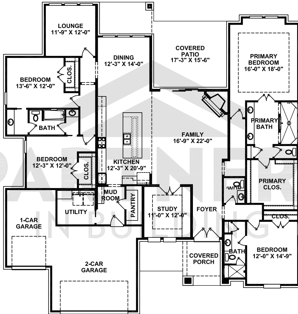
FIRST FLOOR
