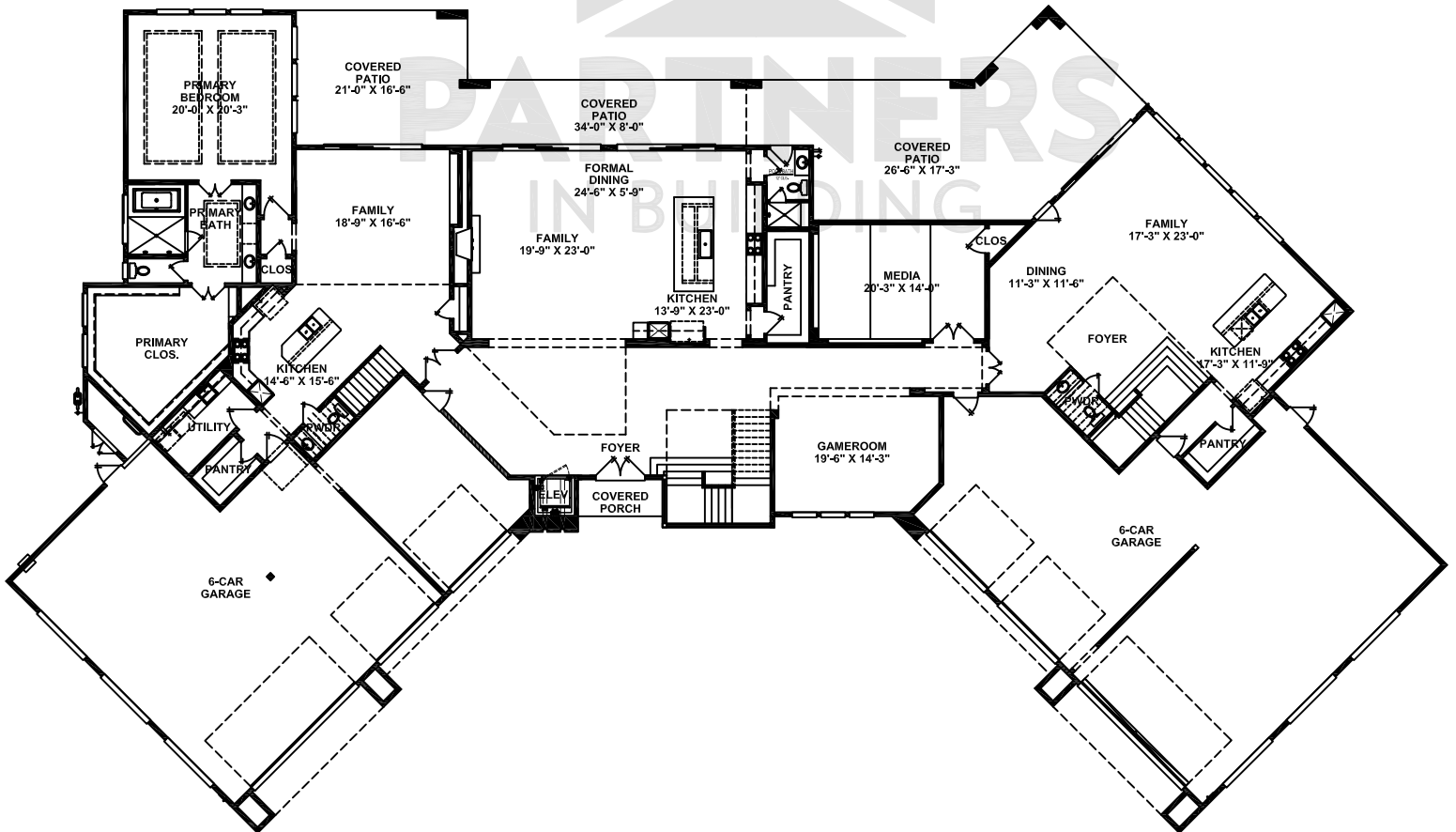
FIRST FLOOR
