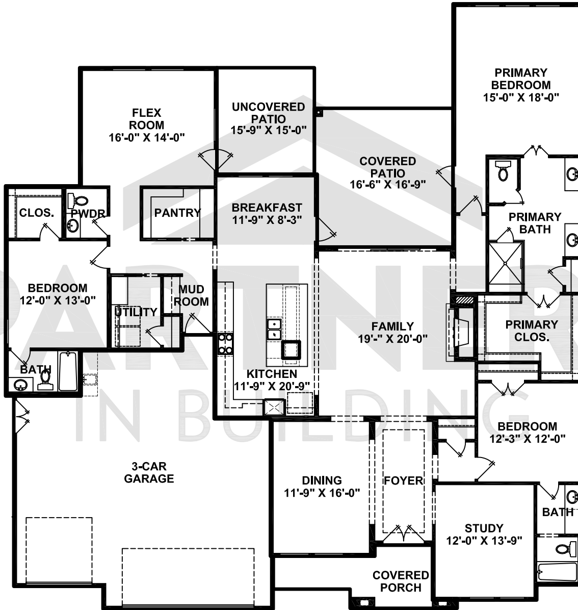
FIRST FLOOR
