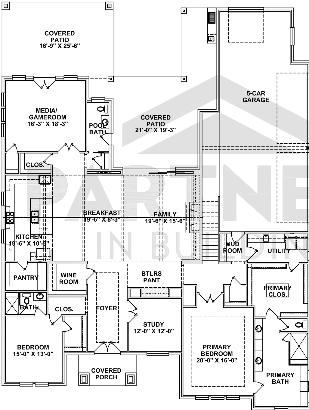
FIRST FLOOR
