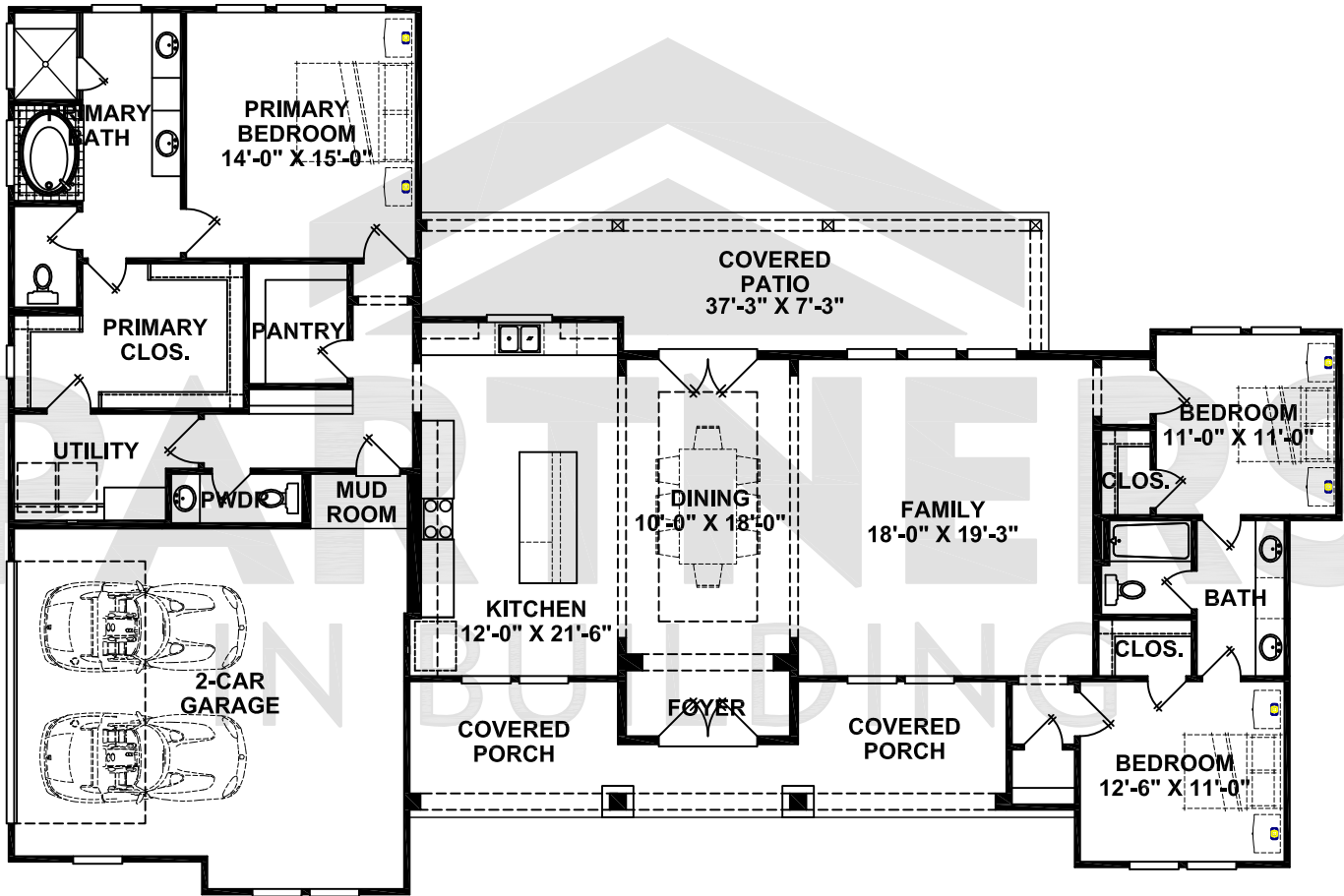
FIRST FLOOR
