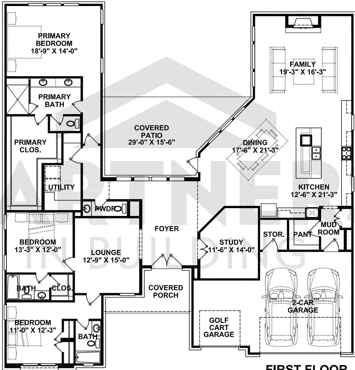
FIRST FLOOR
