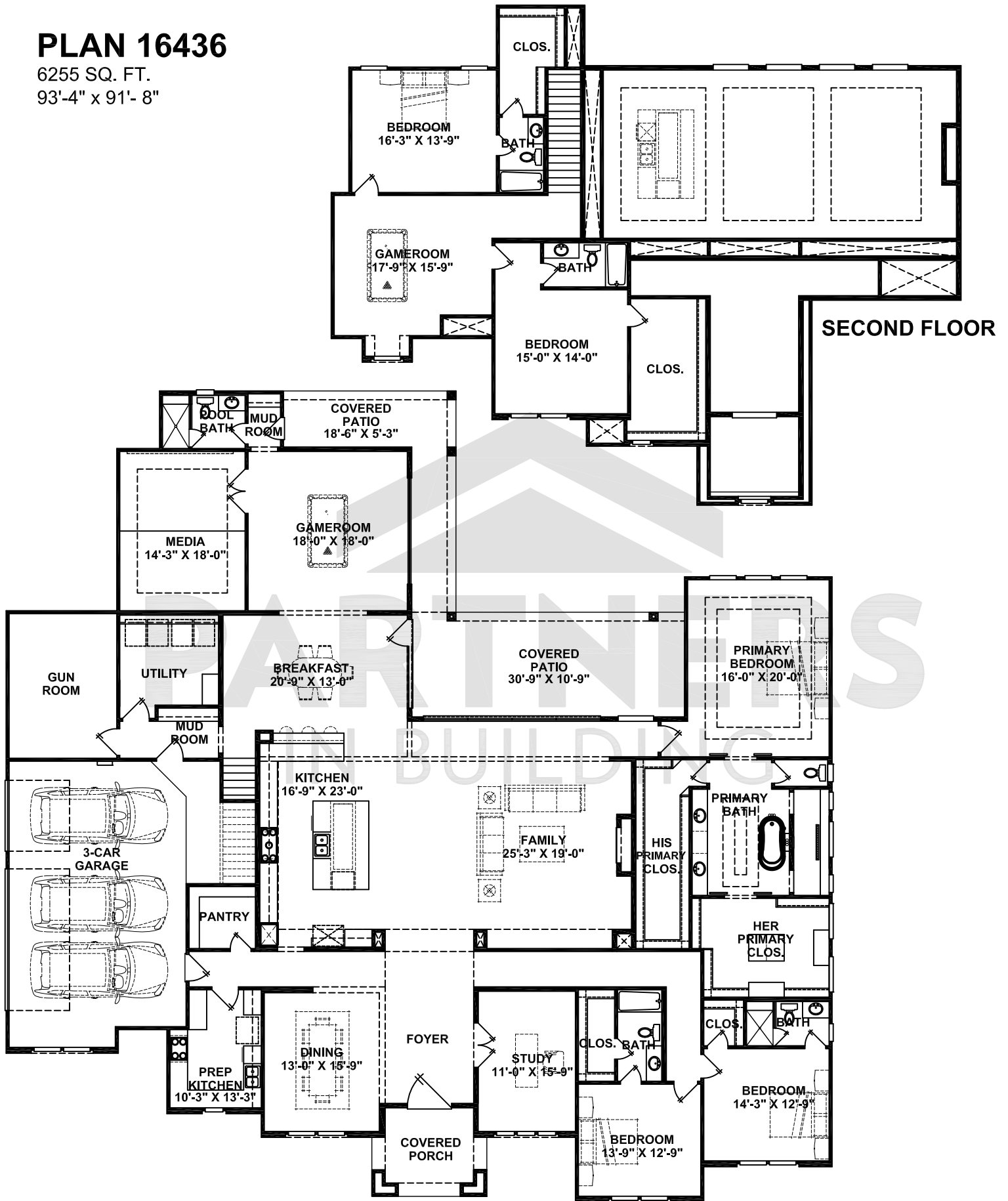
FIRST FLOOR
