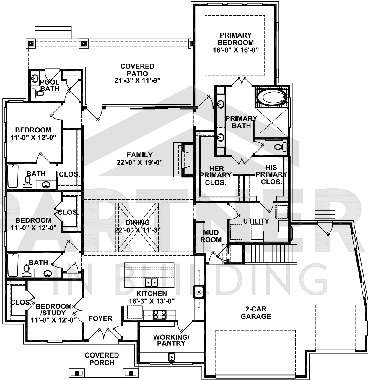
FIRST FLOOR
