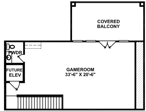
THIRD FLOOR
