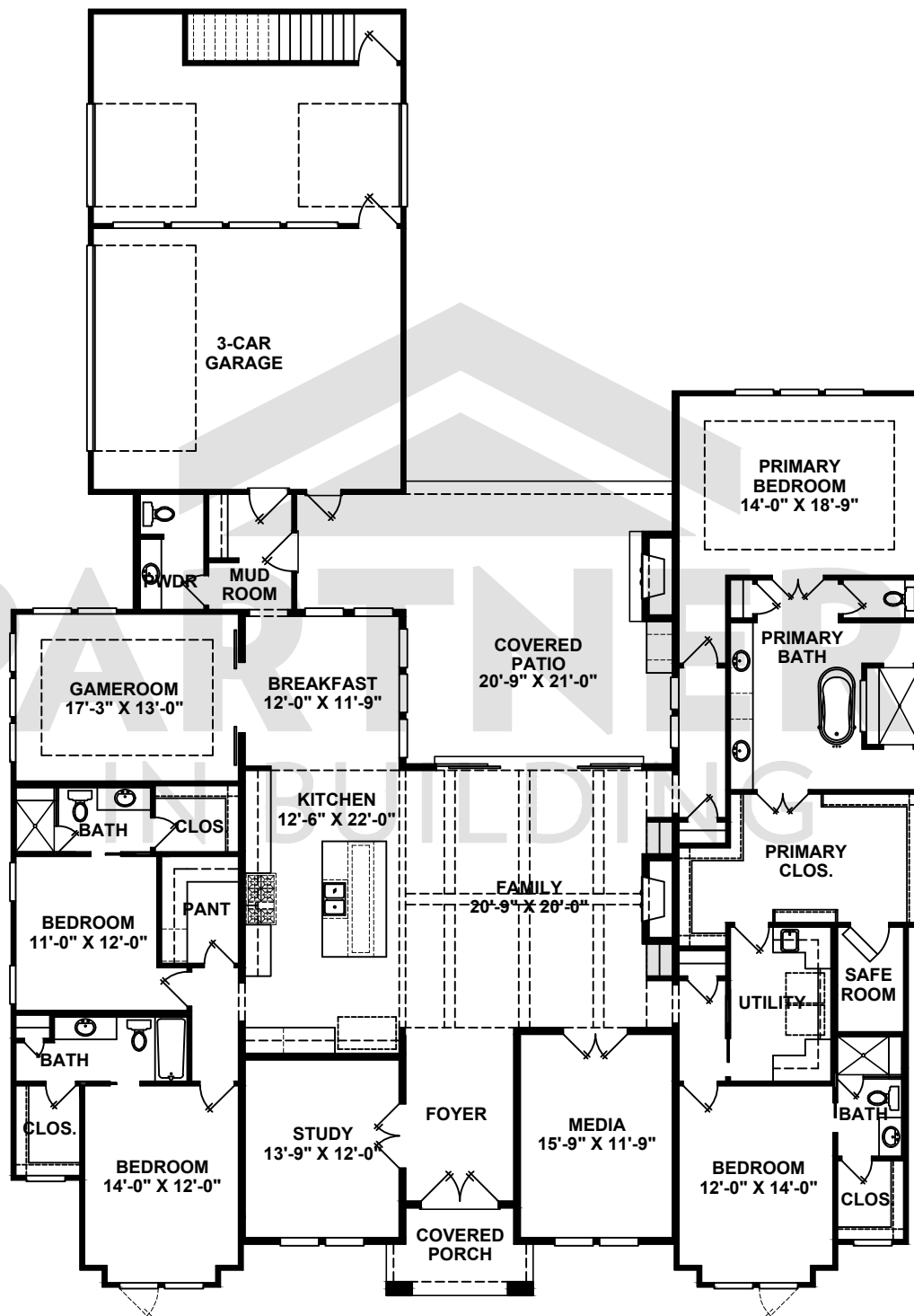
FIRST FLOOR
