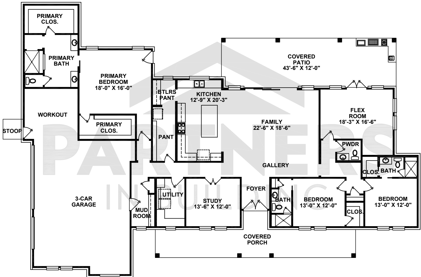
FIRST FLOOR
