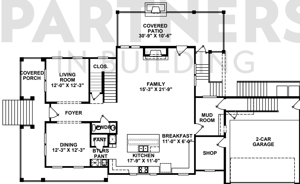
FIRST FLOOR
