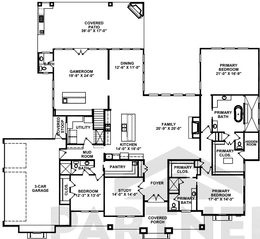
FIRST FLOOR
