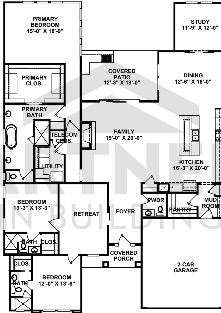
FIRST FLOOR
