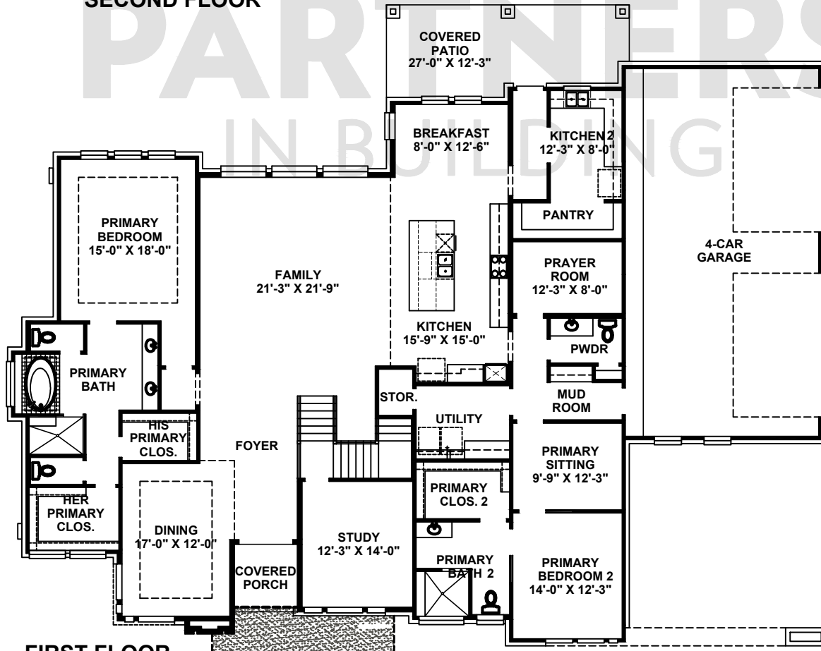
FIRST FLOOR
