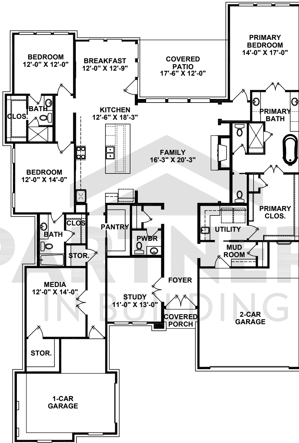
FIRST FLOOR
