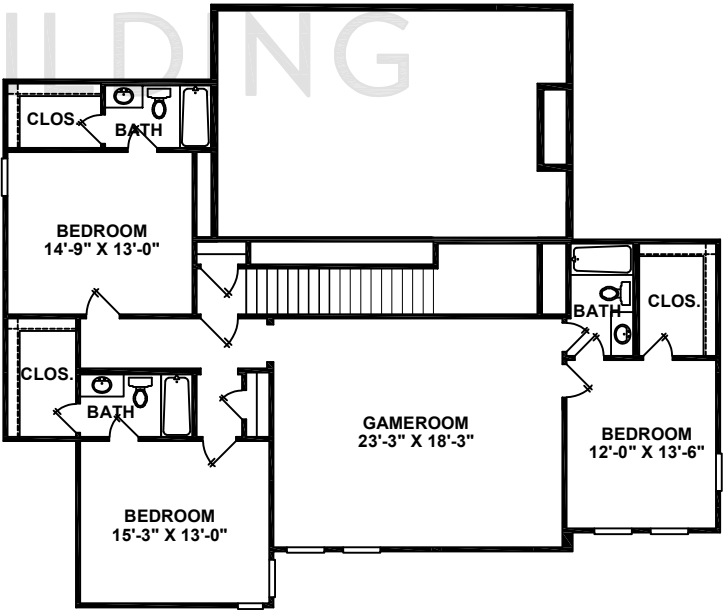
SECOND FLOOR
