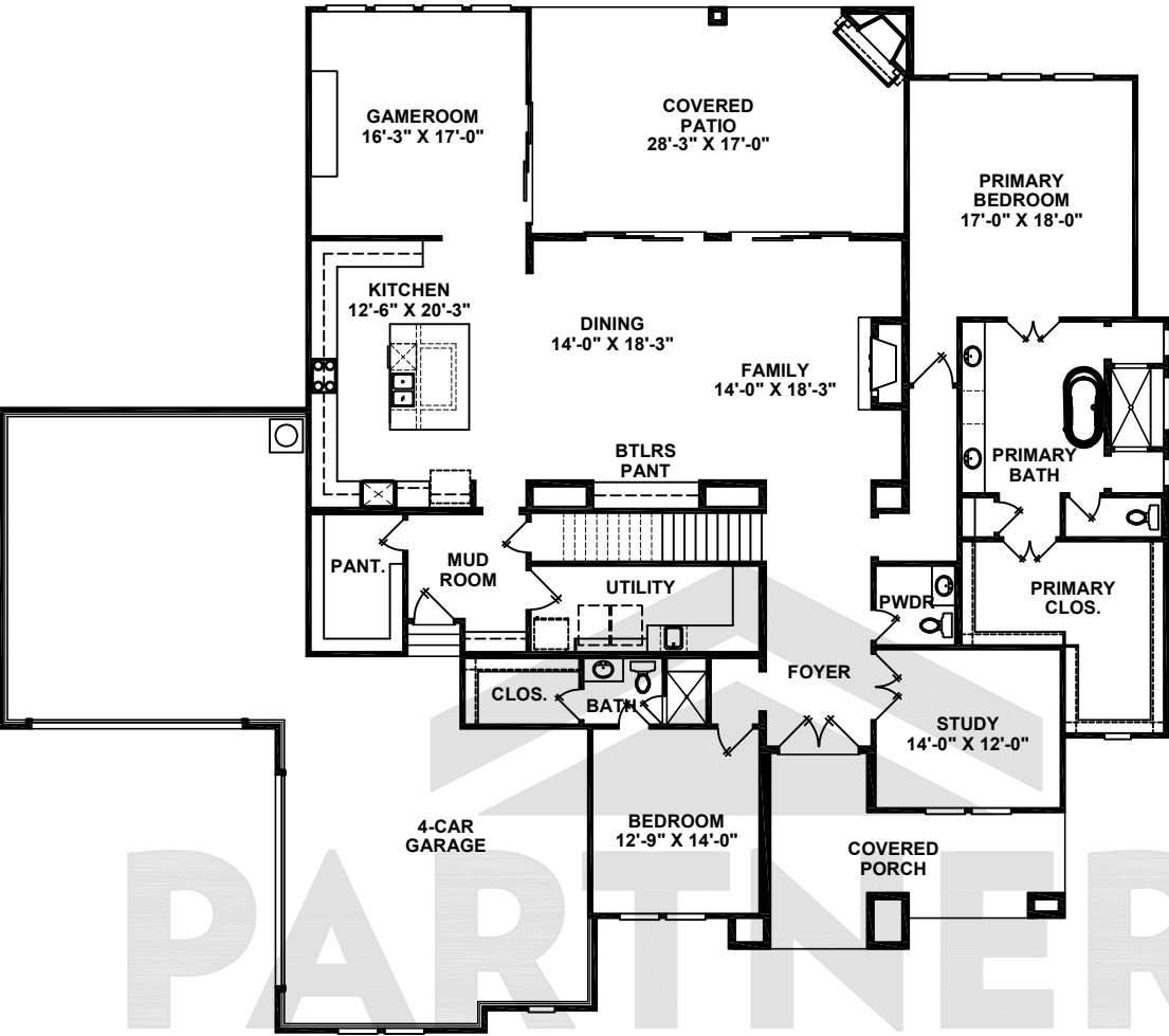
FIRST FLOOR
