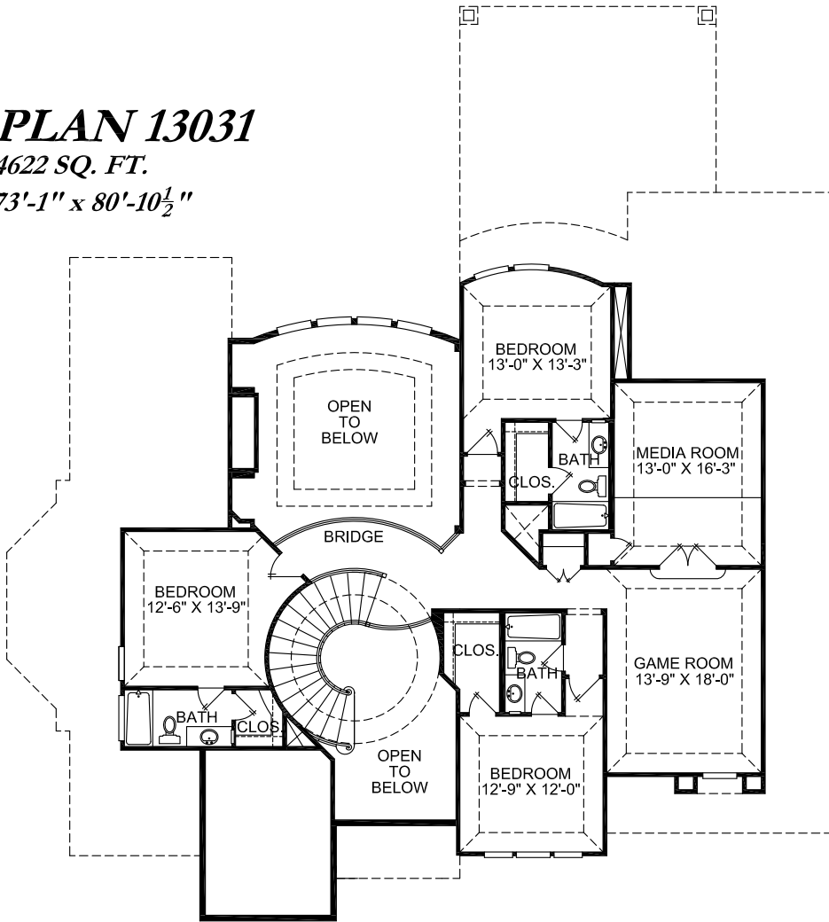
SECOND FLOOR
