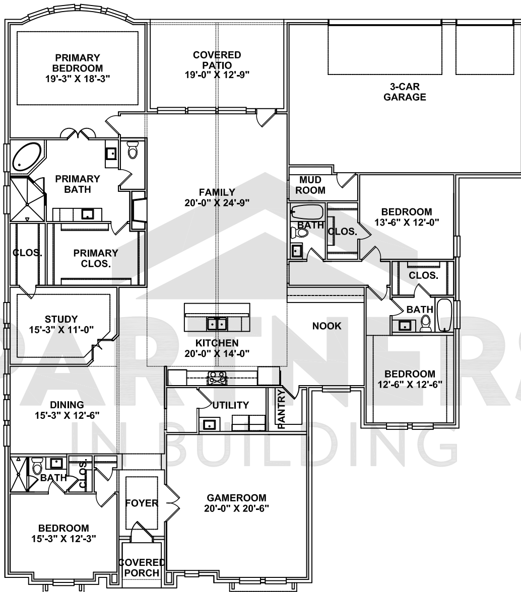
FIRST FLOOR
