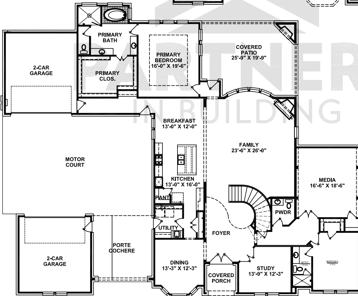
FIRST FLOOR
