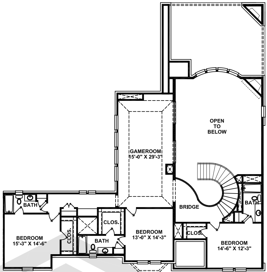
SECOND FLOOR
